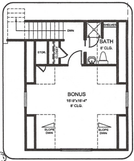
OPTIONAL SECOND FLOOR BONUS ROOM
